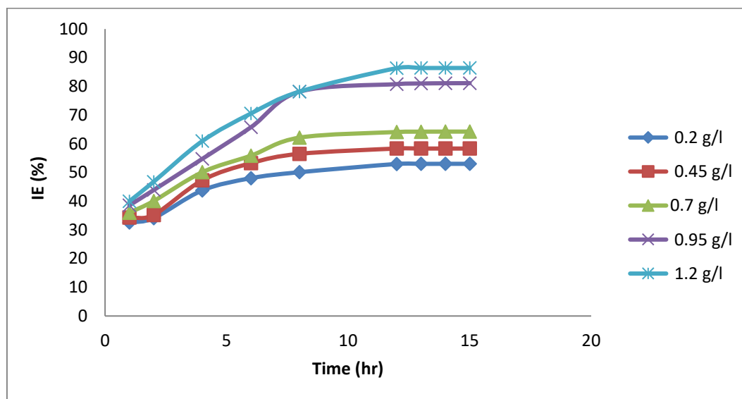
Fig. 2. Plot of IE(%) of zinc in HCl versus time at various concentration of PNL extract.
