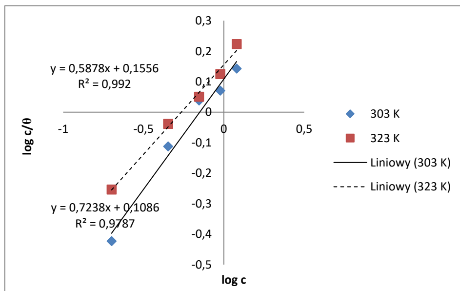
Fig. 3. Plot of Langmuir isotherm for zinc in HCl with PNL extract.
