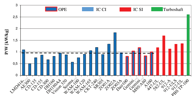
Fig. 14. Power-to-weight ratio for aircraft engines
