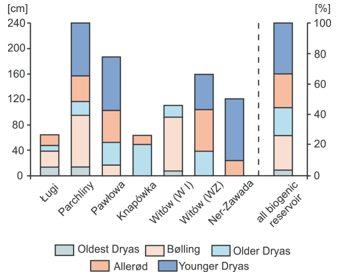
Fig. 9. Rate of calcareous gyttja sedimentation in the Late Weichselian at Ługi (this study); other sites in central Poland according to Wasylikowa (1964, 2011), Kaczmarek (1973), Goździk and Konecka-Betley (1992), Forsysiak et al. (2010), Pawłowski et al. (2016b), and all biogenic accumulation sites
