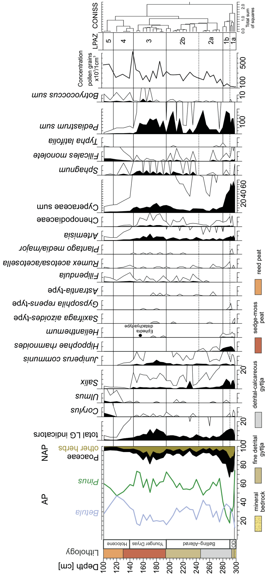
Fig. 3. Percentage pollen diagram from the Lugi peatland, L-1 profile
