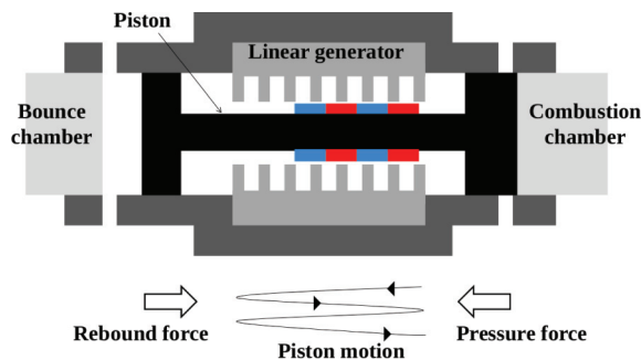
Fig. 1. Schematic of a free piston linear generator
