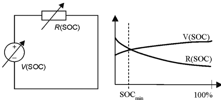
Fig. 2. Battery equivalent circuit
