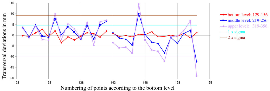
Fig. 12. Results of testing of transversal deviations e_{X_i} of rack poles of the 2 nd track
