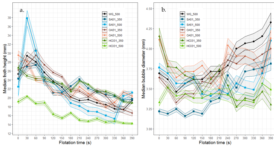
Fig. 6. 30 s median a) froth height and b) bubble diameter in the froth (the ribbons are the 95% confidence interval)
