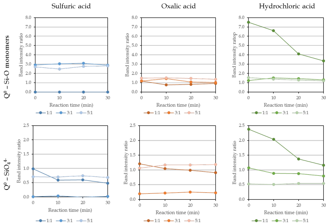
Fig. 15. Evolution of the Raman band intensity ratio of the Q^0 silica species in the mixtures to the Q^0 silica species in pure water glass over the reaction time
