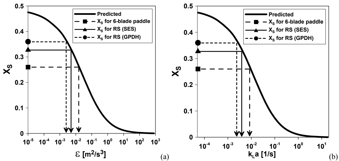
Fig. 14. The results of modelling applied as a calibration curve X_S versus: a) \epsilon , b) k_{La} . The smallest values of the product distribution X_S for three systems considered are applied to present the smallest: a) energy, b) k_{La} , that is required to obtain the measured X_S , (Jasińska et al., 2013b)
