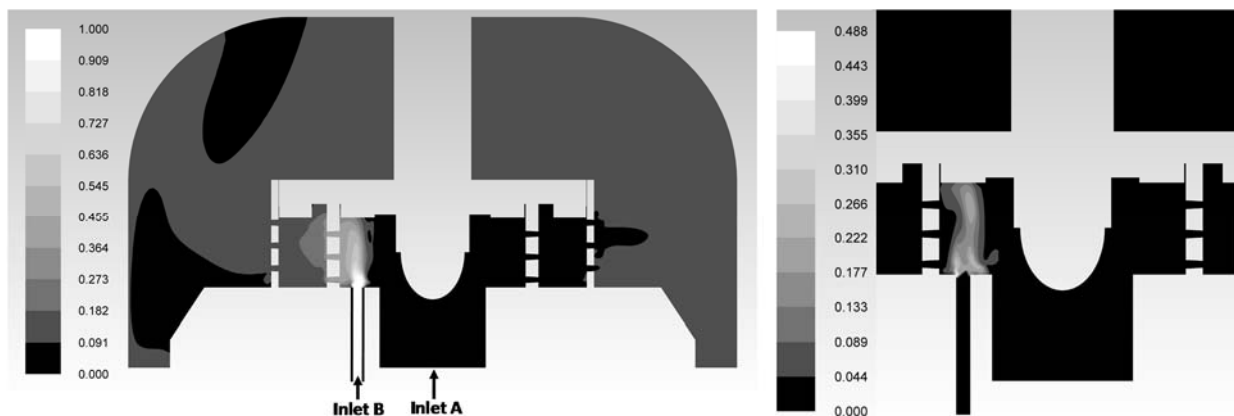
Fig. 8. Results of simulations of mixing in the rotor-stator mixer. Q = 1.0 \times 10^{-4} \text{ m}^3/\text{s} , N = 16.7 \text{ s}^{-1} . a) Mixture fraction distribution, b) Mixture fraction variance distribution. (Jasińska et al., 2013a)
