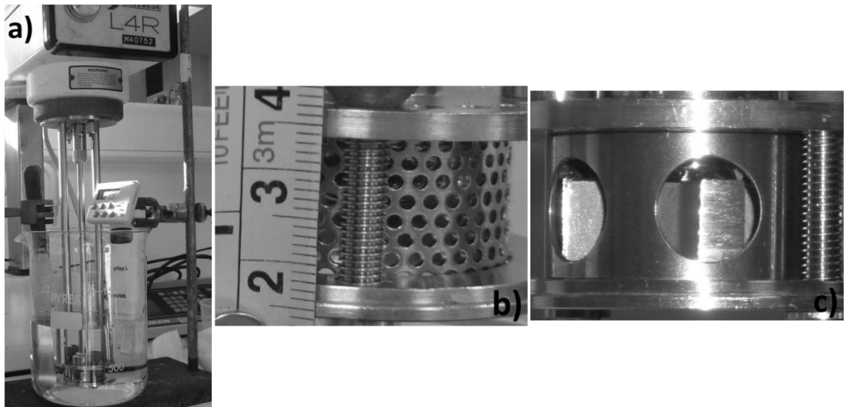
Fig. 11. Experimental setup: a) rotor-stator in batch system, b) standard emulsor screen (SES), c) general purpose disintegrating head (GPDH), (Jasińska et al., 2013b)
