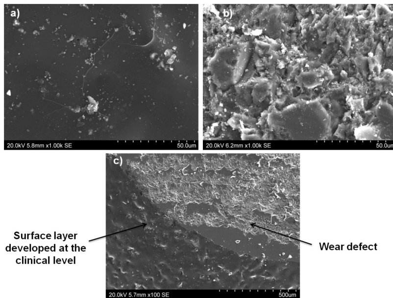
Fig. 12. SEM images of the surface veneered with Vita Titankeramik ceramics on Ti6Al4V incremental sintering substructure: a) surface layer developed at the clinical level, b) surface layer in defects after the wear test, c) border zone between the defects and the area before the wear test
