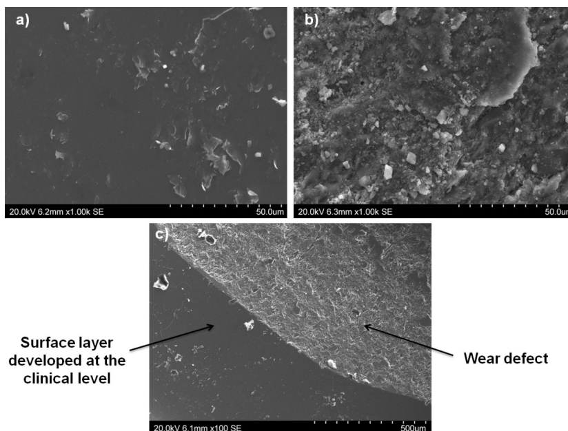
Fig. 13. SEM images of the surface veneered with IPS e.max Ceram ceramics on the milled \text{LiSi}_2 substructure: a) surface layer developed at the clinical level, b) surface layer in the defect after the wear test, c) border zone between the defect and the area before the wear test
