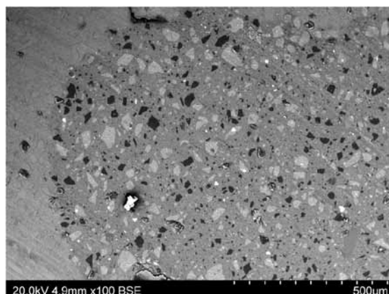
Fig. 6. SEM image of wear defect edge in the Essentia material
