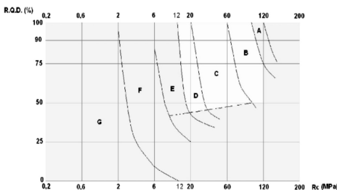
Fig. 2. Efficiency of using vibration rippers when compared to hydraulic hammers [L. 2, 6]
