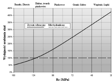
Fig. 2. Efficiency of using vibration rippers when compared to hydraulic hammers [L. 2, 6]
