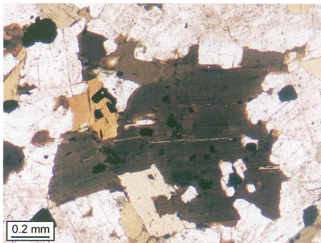
Fig. 11. Red-brown biotite in granodiorite (transition zone), borehole DB-5, depth 1370.0 m. Plane-polarized light
