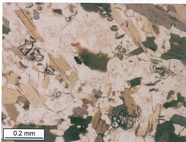
Fig. 7. Euhedral and subhedral corundum crystalloblasts in dark micaceous enclave, borehole DB-5, depth 1370.0 m. Plane-polarized light
