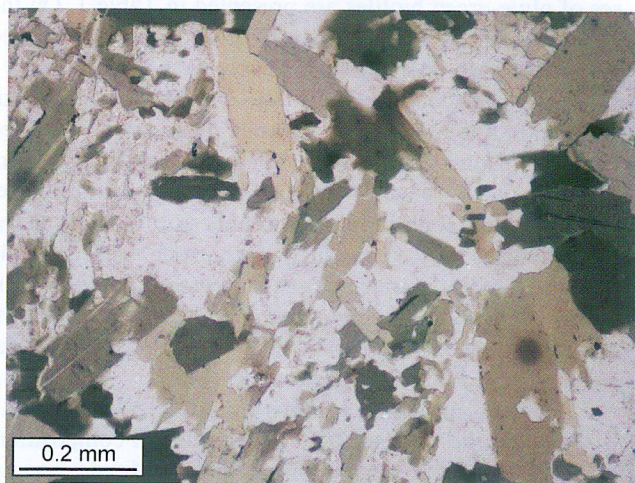
Fig. 8. Olive-green biotite in dark micaceous enclave (transition zone), borehole DB-5, depth 1370.0 m. Plane-polarized light
