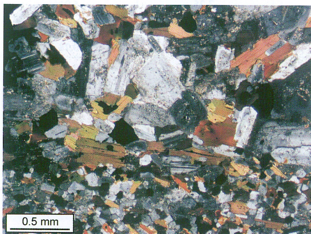
Fig. 9. Plagioclase plates and biotite flakes arranged parallel to the boundary of dark micaceous enclave and granodiorite from Będkowska Valley, borehole DB-5, depth 1370.0 m. Crossed polars
