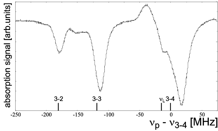
Fig. 3. Absorption, wide scan over all hfs components. The trapping laser is at \nu_L = \nu_{3-4} - 12 MHz. Intensity of each trapping beam is 14.4 \text{ mW/cm}^2 .
