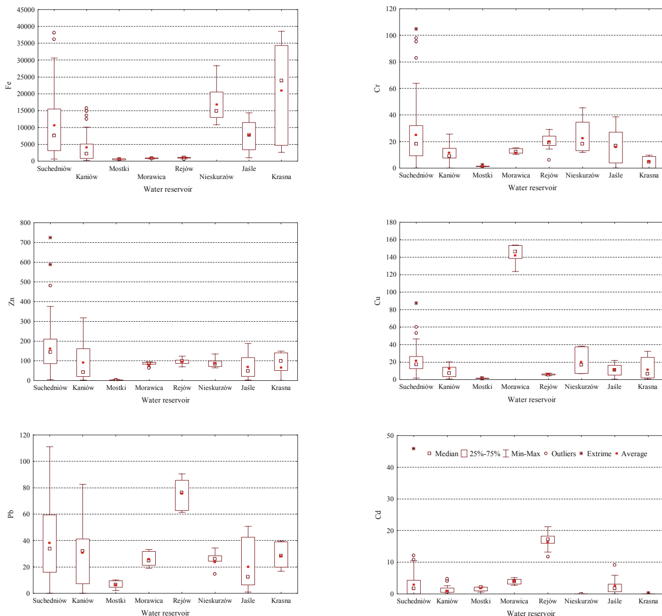
Fig. 3. Trace metal concentrations [ \text{mg}\cdot\text{kg}^{-1} ] in the sediments of examined water reservoirs
