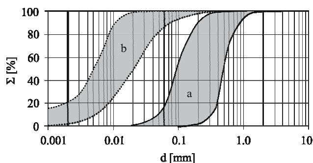
Fig. 2. Boundaries of granulometric curves of bottom sediments: a – collected from upper part of examined water bodies; b – collected from lower part of examined water bodies
