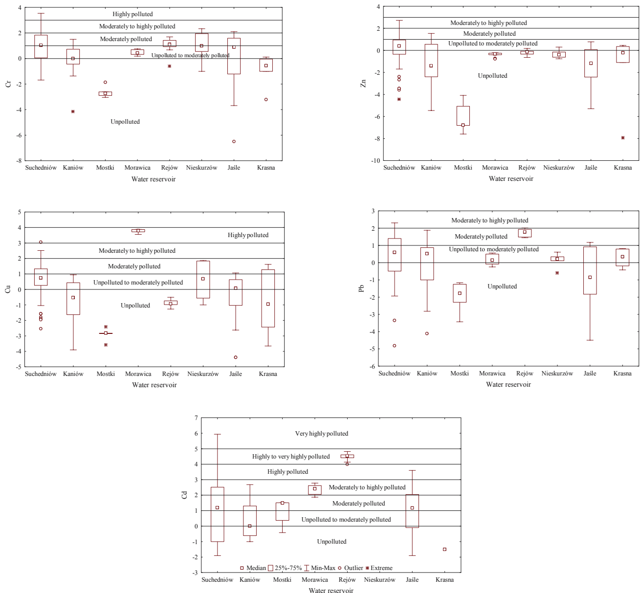
Fig. 6. Box plot of I_{geo} for the studied elements in investigated water reservoirs
