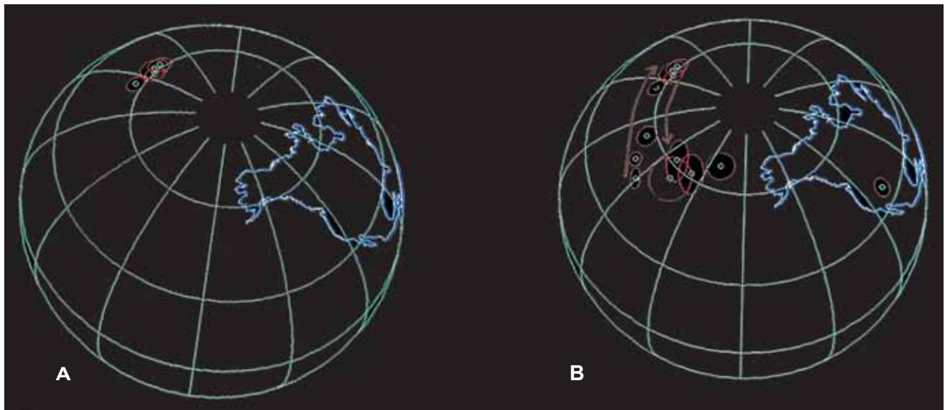
Fig. 6. Whitmore Point paleopoles and Mesozoic APW
