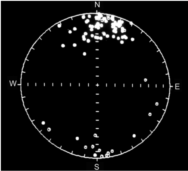
Fig. 4. All thermally demagnetized data from the Whitmore Point Member
