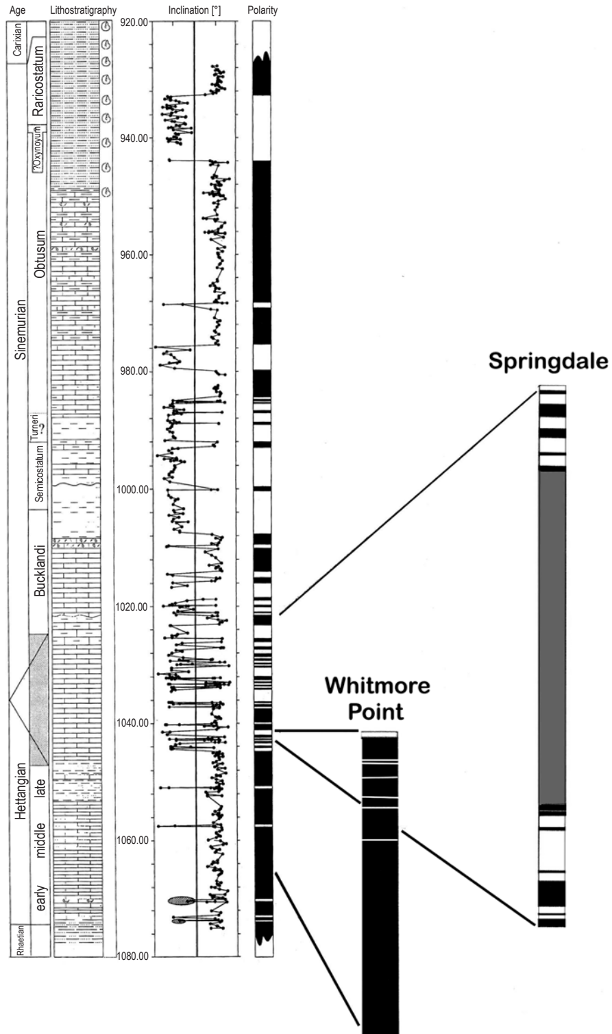
Fig. 5. Comparison between the paleomagnetic polarity from the Hettangian and Sinemurian of the Paris Basin (after Young et al. , 1996) and the Whitmore Point and Springdale magnetostratigraphy
