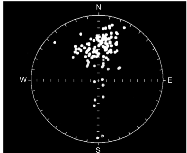
Fig. 3. Directions of natural remanent magnetization, equal-area projection
