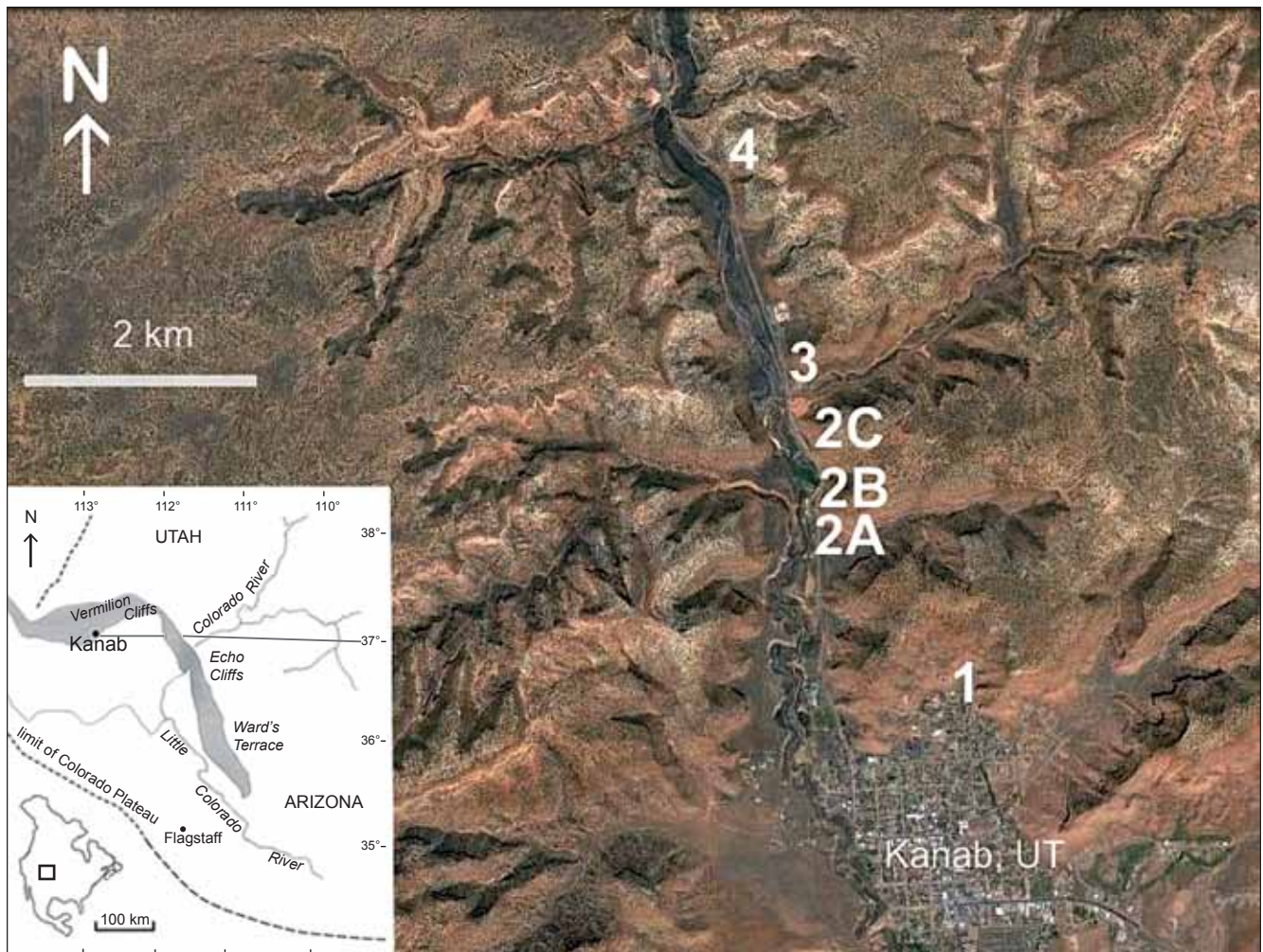
Fig. 1. Location map, showing the sampling sites near Kanab
