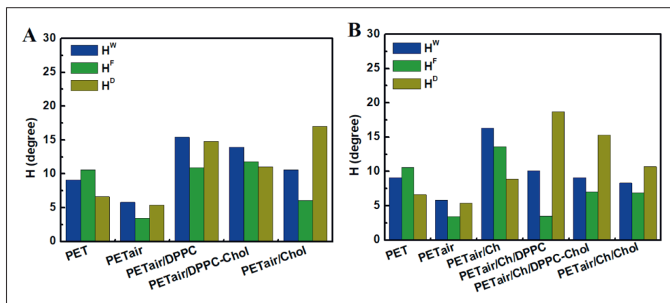
Figure 2. Contact angle hysteresis of water( H^W ) formamide( H^F )and diiodomethane( H^D )calculated for the unmodified commercial and modified polyethylene terephthalate (PET) surfaces (A)without and (B) with a chitosan (Ch) layer
