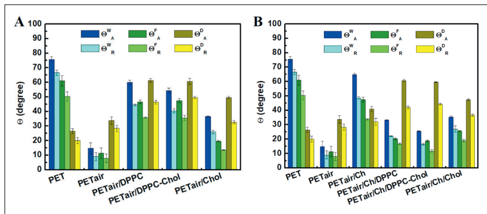
Figure 3. Contact angles of water (W), formamide (F) and diodomethane (D) measured on the unmodified commercial and modified polyethylene terephthalate (PET) surfaces (A) without and (B) with a chitosan (Ch) layer
