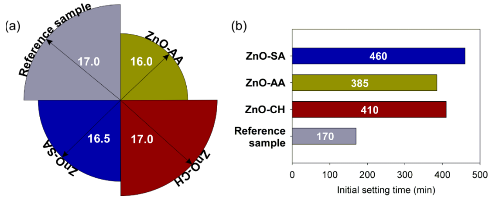
Fig. 2. Plasticity (a) and the initial setting time (b) of mortars
