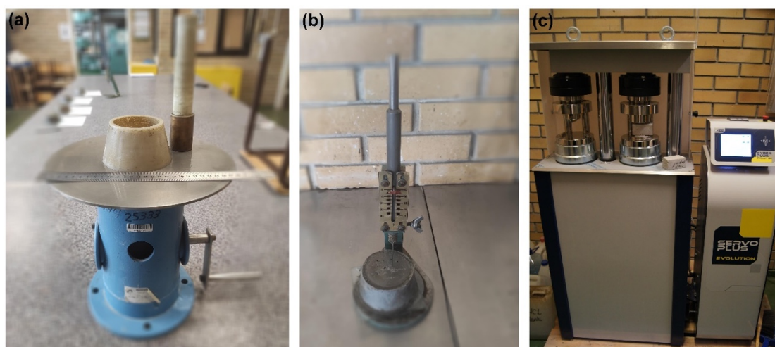
Fig. 1. Digital images of basic equipment used in the study: flow table (a), Vicat apparatus (b) and testing press machine (c)
