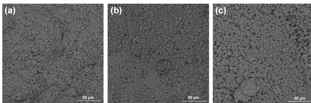
Fig. 6. SEM images of cement composites doped with ZnO-CH (a), ZnO-AA (b) and ZnO-SA (c)
