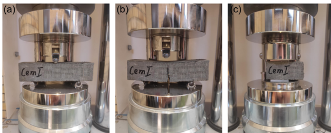
Fig. 5. Digital images of cement mortar during (a) and after (b) flexural strength test and sample during compressive strength test (c)
