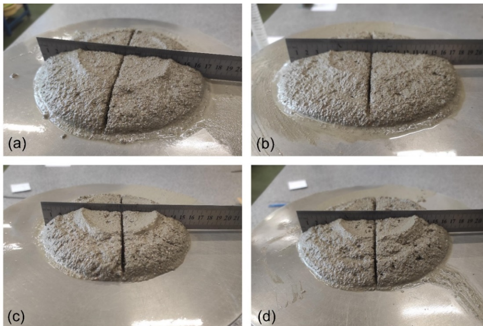
Fig. 3. Digital images of cement mortars during plasticity testing without (a) and with ZnO-CH (b), ZnO-AA (c) and ZnO-SA (d) admixtures
