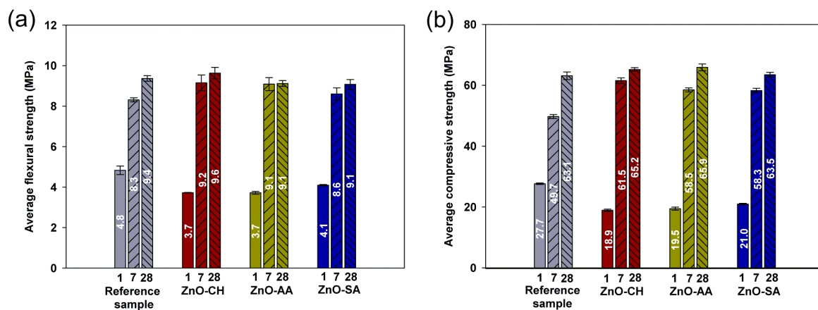
Fig. 4. Average flexural (a) and compressive (b) strength of cement mortars after 1, 7 and 28 days maturation
