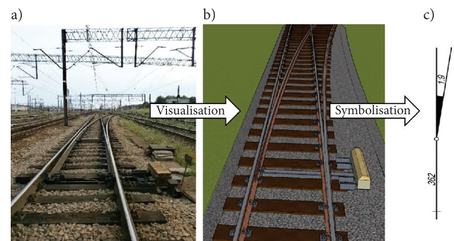
Fig. 2. The process of coding of a regular electric turnout Rz S60 – 1:9 – 300: a) real object [photography of authors], b) visualised model (concept) [drawing of authors], c) cartographic symbol, GK-1 code: RZE; own elaboration based on [5]
