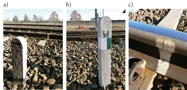
Fig. 4. Stabilised fixed points of reference for observing the areas susceptible to creep of rails in a continuous welded track: a) fixed to a concrete post – rear view [photography of authors], b) fixed to a concrete post – front view. Markings according to Id-1 (D-1) [photography of authors], c) base point – a notch in the external surface of the railhead [photography of authors]
