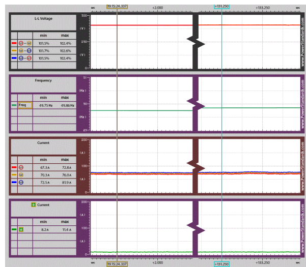
Fig. 6. Under-frequency event during drive operation
