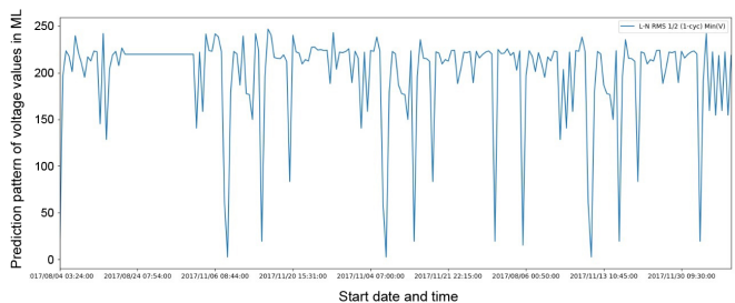
Fig. 11. FDIPA training outcome with respect to past data analysis
