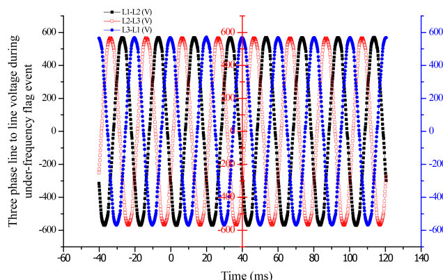
Fig. 7. Under-frequency signal patterns during drive operation
