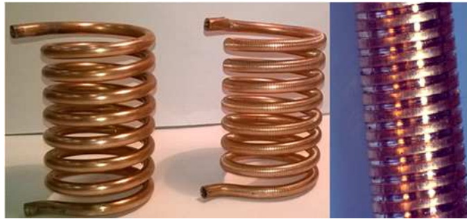
Figure 3: Obtained construction of helical coils: at the left side – coil made from smooth copper pipe, in the middle – coil with modified surface, at the right side – photo of modified surface.
