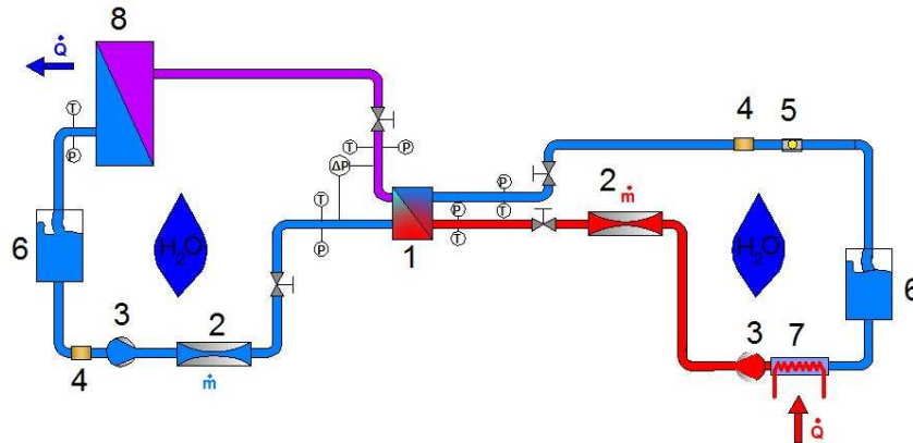
Figure 4: Schematic diagram of experimental rig: 1 – helical coil heat exchanger, 2 – Coriolis mass flow meter, 3 – non-pulsation gear pump, 4 – filter, 5 – inspection glass, 6 – fluid tank, 7 – heater, 8 – chiller.
