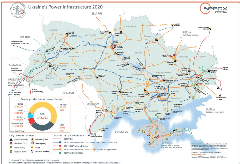
Fig 1. The United energy system of Ukraine
