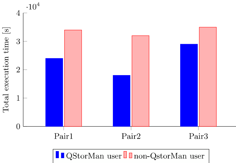
Figure 4. Execution time of application with and without QStorMan support
