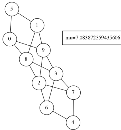
Figure 14. A counterexample for the conjectured bound \mu \leq \max_v m_v \sqrt{1 + \frac{3m_v}{d_v}} .
