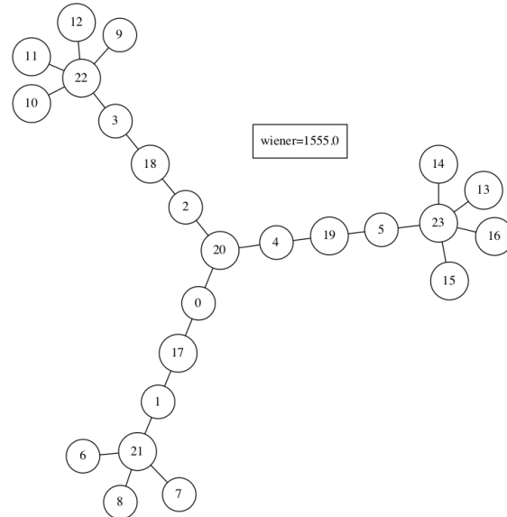
Figure 6. Tree on 24 vertices with the maximum Wiener index and radius 5.
