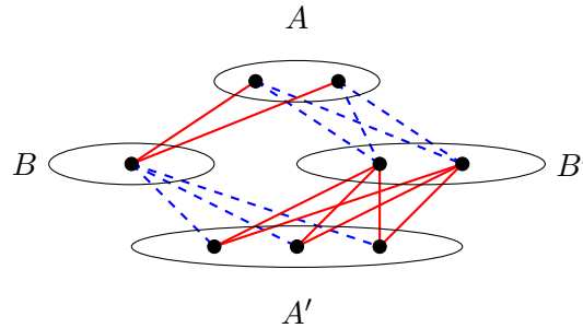
Figure 7. A properly connected 2-coloring of K_{3,5} with proper diameter 4.
