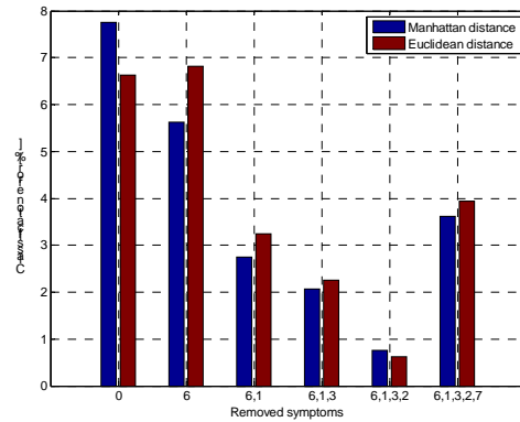
Fig. 3. Changes of classification error in consecutive steps of rejecting useless symptoms (0 means that no symptom was rejected)
