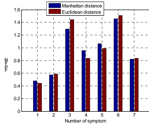
Fig.2. FP/FN ratio for single-symptom-classifiers k -NN with weighted voting
