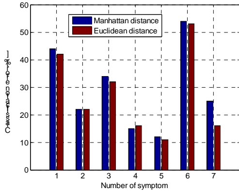
Fig.1. Classification errors for single-symptom-classifiers k -NN with weighted voting
