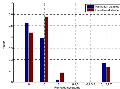
Fig. 4. Changes of the FP/FN ratio in consecutive steps of rejecting useless symptoms (0 means that no symptom / parameter was rejected)
