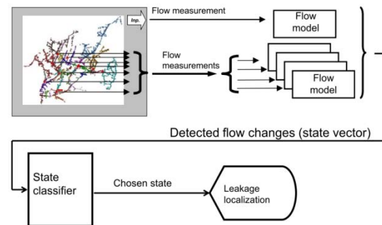
Fig. 7. A scheme of a leakage location method [30]
