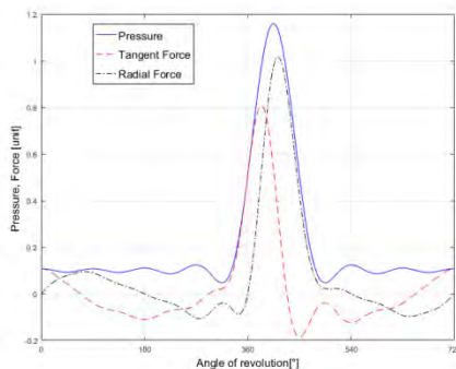
Fig. 2. Expanded indicator diagram of the studied engine.
