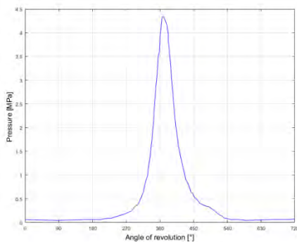
Fig. 1. Indicator diagram.4
