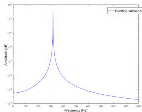
Fig. 8. Bending vibrations of the crankshaft of the system without coupling.
