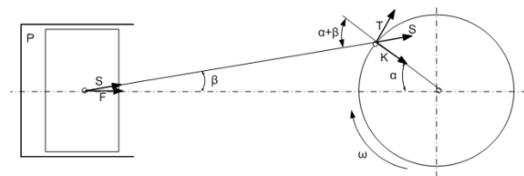
Fig.3. The diagram presenting the distribution of forces in the crank-piston mechanism.
