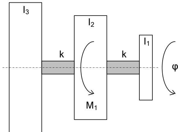
Fig. 4. Shaft model.
