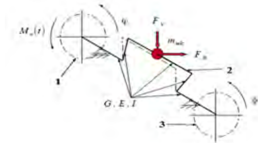
Fig.6. Model of the crankshaft
