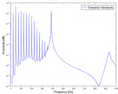
Fig. 5. The amplitude of torsional vibration acceleration of the model
