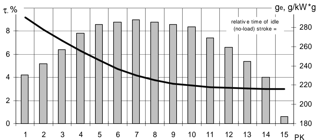
Fig. 1. Consumption characteristic of Diesel-generator 1A-9DG and distributing of under-load operation conditions of diesel locomotive power-plant: \tau – relative time of operation of the DG; ПК – position of controller-engine-driver
