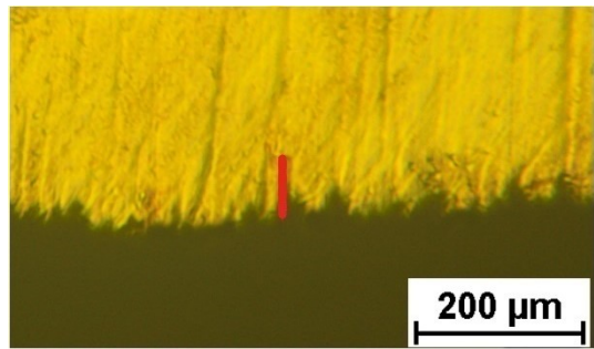
Fig. 20. The image of the surface layer of CuZn37As0.033 alloy. Dezincification 85μm
