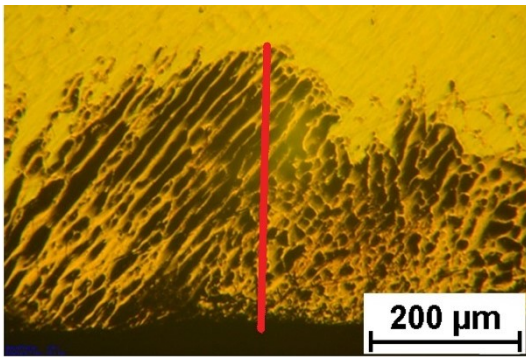
Fig. 16. The image of the surface layer of CuZn37Al0.75 alloy. Dezincification 400μm
