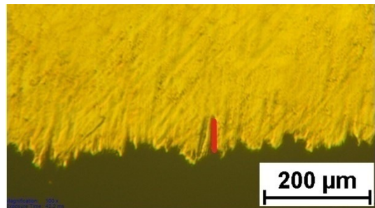
Fig. 21. The image of the surface layer of CuZn37As0.055 alloy. Dezincification 65μm
