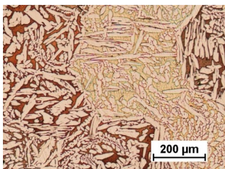
Fig. 8. The microstructure of MS-60 alloy, the casting from the OBB Sand mould obtained from the charge in the form of ingots
