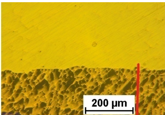
Fig. 19. The image of the surface layer of CuZn37Sn1.24 alloy. Dezincification 225μm
