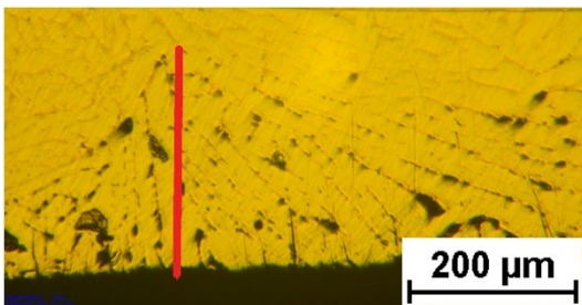
Fig. 17. The image of the surface layer of CuZn37Al1.21 alloy. Dezincification 290μm
