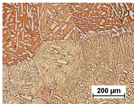
Fig. 10. The microstructure of MS-60 alloy, the casting from the wet sand mould obtained from the charge in the form of pigs
