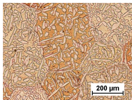
Fig. 11. The microstructure of MS-60 alloy, the casting from the OBB Sand mould obtained from the charge in the form of pigs
