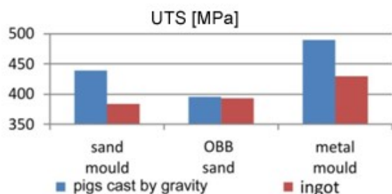
Fig. 13. The tensile strength results of the samples made of MS-60 alloy
