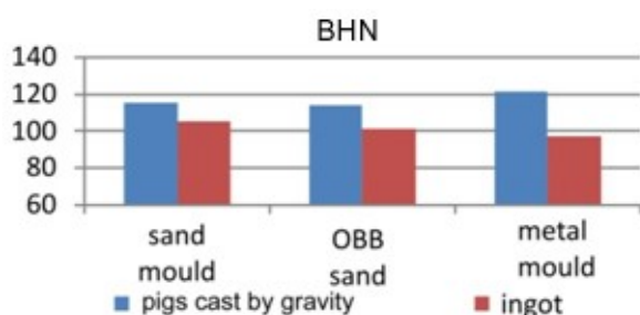
Fig. 14. The results of the hardness tests of the samples made of MS-60 alloy
