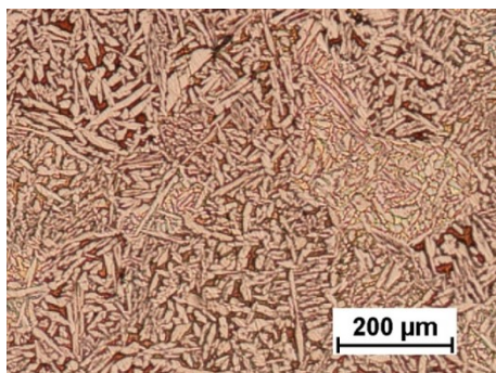
Fig. 9. The microstructure of MS-60 alloy, the casting from the metal mould obtained from the charge in the form of ingots
