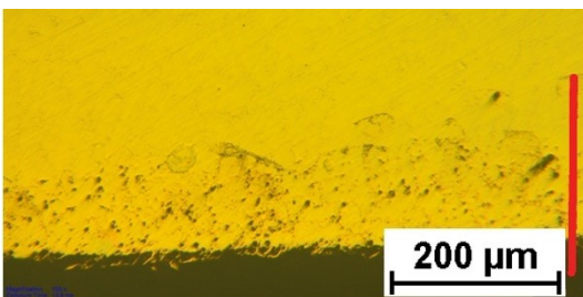
Fig. 18. The image of the surface layer of CuZn37Sn0.71 alloy. Dezincification 240μm
