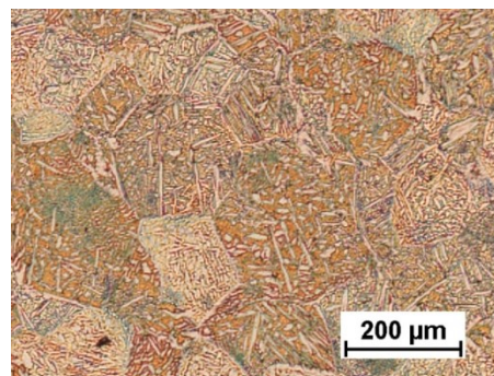
Fig. 12. The microstructure of MS-60 alloy, the casting from the metal mould, obtained from the charge in the form of ingots cast by gravity
