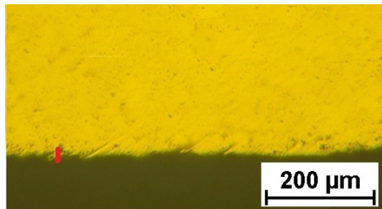
Fig. 22. The image of the surface layer of CuZn37As0.37 alloy. Dezincification 20μm
