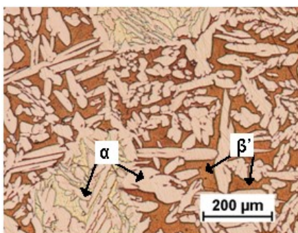
Fig. 7. The microstructure of MS-60 alloy, the casting from the wet sand mould obtained from the charge in the form of ingots
