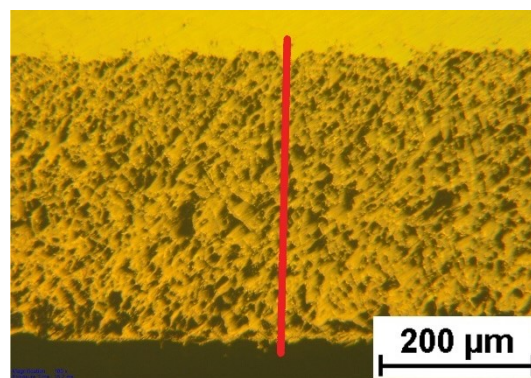
Fig. 15. The image of the surface layer of CuZn37Al0.001 alloy. Dezincification 450 \mu\text{m}
