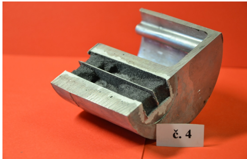
Fig. 6. H 2400 during dissolution of the glued core
