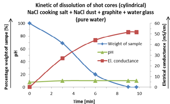
Fig. 9. Kinetics of dissolution of salt cores in dependence on pH and electric conductance
