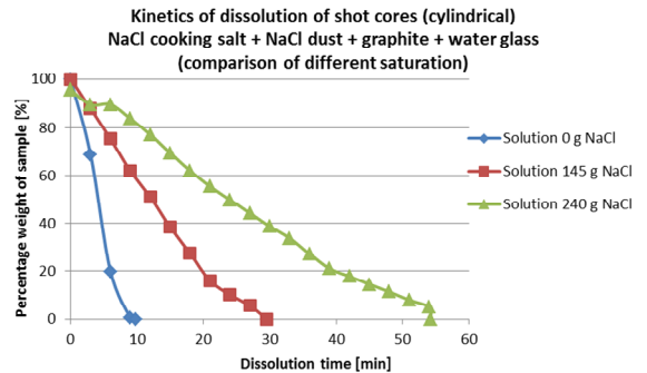
Fig. 8. Comparison of dissolving the salt cores in two types of saturated solutions and in pure water
