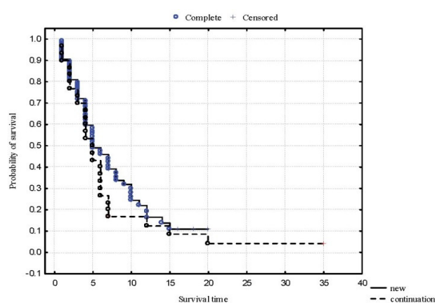
Figure 2 Kaplan-Meier survival estimates (CONTINUATION vs. NEW)
