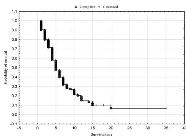
Figure 1 Kaplan-Meier survival estimates (full sample)
