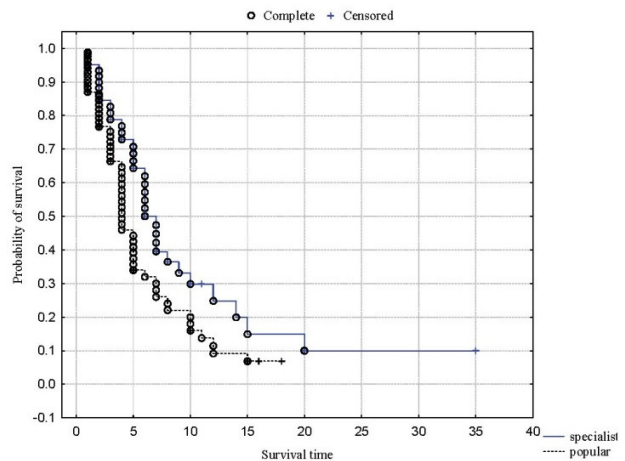
Figure 6 Kaplan-Meier survival estimates (POPULAR vs SPECIALIST)
