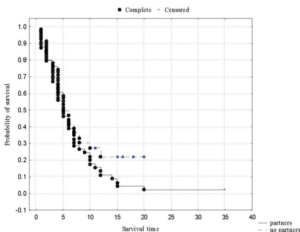
Figure 3 Kaplan-Meier survival estimates (PARTNERS vs NO PARTNERS)
