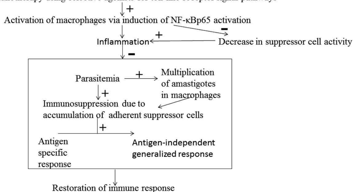
Fig. 3. Mode of action of toll-like receptor agonists in reversal of Leishmania parasite-induced immunosuppression. Mechanism of toll-like receptor agonists in reversal of immunosuppression via down regulation of adherent suppressor cells causing antigen specific and independent generalized immunosuppression during progression of disease. The increase in parasitemia gradually shifts antigen specific suppression of lymphoproliferative response to generalized antigen independent response in susceptible population. Removal of adherent cells restores functional immune response. The “+” sign indicates increase while the “-” sign indicates decrease in response.
