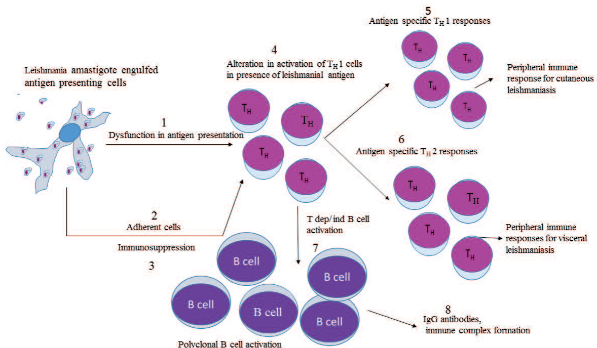
Fig. 2. Multifunctional immune responses following infection of leishmania parasites. Intracellular growth and multiplication of Leishmania parasites develop alteration in functional immune responses in immunocompetent hosts. There are different steps in antigen specific immune responses, alteration in any or more than one stage generate dysfunction in protective immune response to prevent infection. 1. Dysfunction in antigen presentation by antigen presenting cells; 2. Presence of adherent cells having suppressor cell property; 3. T-helper cell (T H )-dependent immune responses include antigen specific and generalized immunosuppression); 4. Alteration in activation of T H 1 cells; 5. Antigen specific T H 1 cell responses; 6. Antigen specific T H 2 cell responses; and 7. T dependent as well as independent B cell activation. The polyclonal B cell activation and T cell-mediated peripheral immune responses are found during progression of leishmaniasis.
