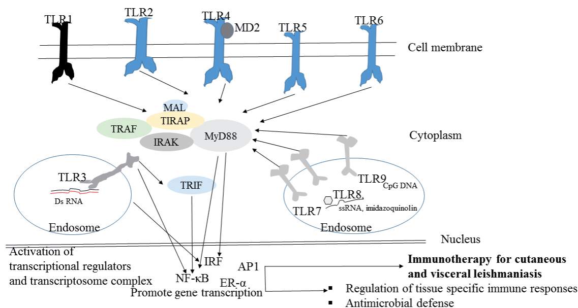
Fig. 1. Signal events of extracellular TLR 2, 4, 5, 6 and intracellular TLR 3, 7, 8, 9. The extracellular and intracellular toll-like receptors (TLRs) induce signals through activation of MyD88 adaptor protein and intermediate MAL/TIRAP, TRAF, IRAK signal adaptor protein molecules. The TLR3 signal pathway includes TRIF. The TLR-mediated signals differentially induce downstream activation of NF- \kappa B, AP1, ER- \alpha and IRF to promote gene expressions. The immunotherapy of cutaneous and visceral leishmaniasis depends on selective activation of TLR-signals for regulation of tissue specific immune responses and antimicrobial defense.
