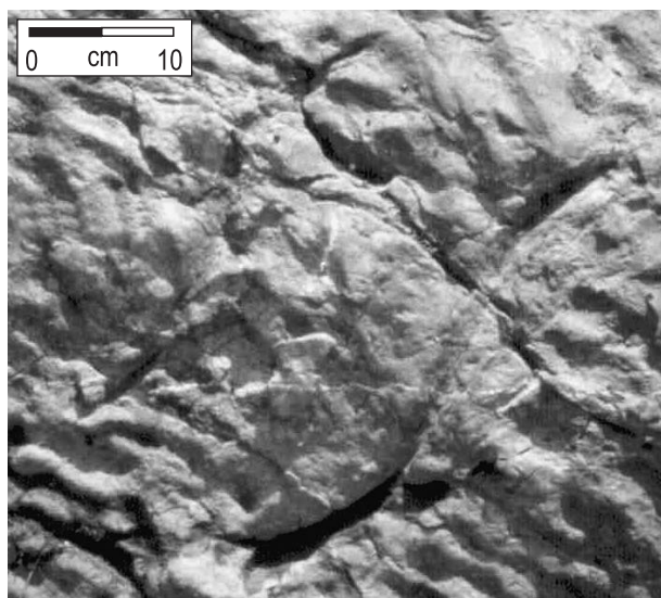
Fig. 31. Scratches in lacustrine sediments of the Early Cretaceous Cameros Basin (Rioja, Spain), ascribed to the claws of a dinosaur that was unintentionally swimming. Photo Loïc Costeur (Nantes).
