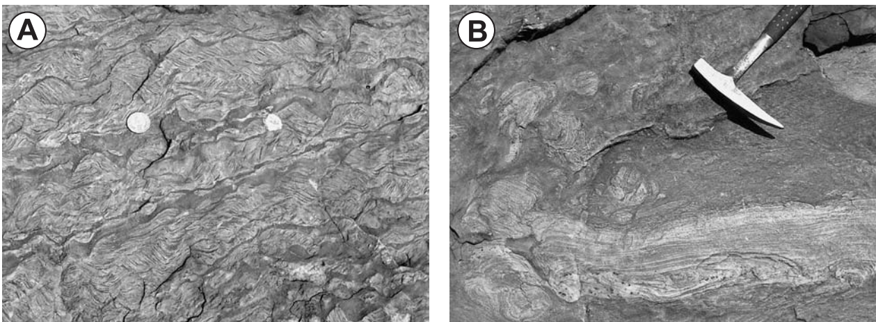
Fig. 2. Complex deformations. A: Complex deformations that are typical of silt-rich layers. Palaeoproterozoic succession affected by seismic shocks (seismites) near Dhalbhum Gar (India). B: Complex deformation due to deformation of an earlier deformed layer: a layer with probably shock-induced deformations (e.g., loadcasts) underwent mass transport that resulted in a slump head. Palaeoproterozoic Chaibasa Fm. (Singhbhum area, E India).
