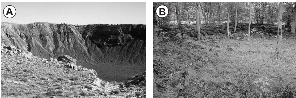
Fig. 13. Impact structures. A: The crater wall of Meteor Crater (Arizona, U.S.A.), seen from the opposite crater wall. B: A small ring-wall surrounding a depression formed by the impact of a piece of an exploded meteorite in a thin glacial cover on top of Devonian carbonates near Kaali (Estonia). Photo W. Stankowski (Poznań).
