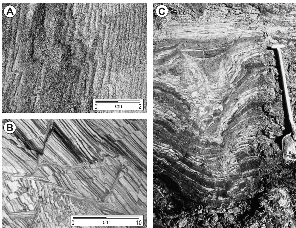
Fig. 8. Complex deformations. A: Kink structures (originally considered as characteristic of crystals - later of crystals and lithified rocks only - in ice-pushed glaciofluvial sands, Bełchatów opencast browncoal mine (central Poland). B: Shear plains genetically related to kink structures in glacitectonically disturbed fluvioglacial sands near Farlebjergus (Denmark). C: Fairly complex gravifossium (essentially due to reversed density gradients, but see caption of Fig. 7B), formed between 1200 and 1600 AD, near Emmeloord (The Netherlands) in the fine-grained lagoonal Almere Member of the North Sea Formation.
