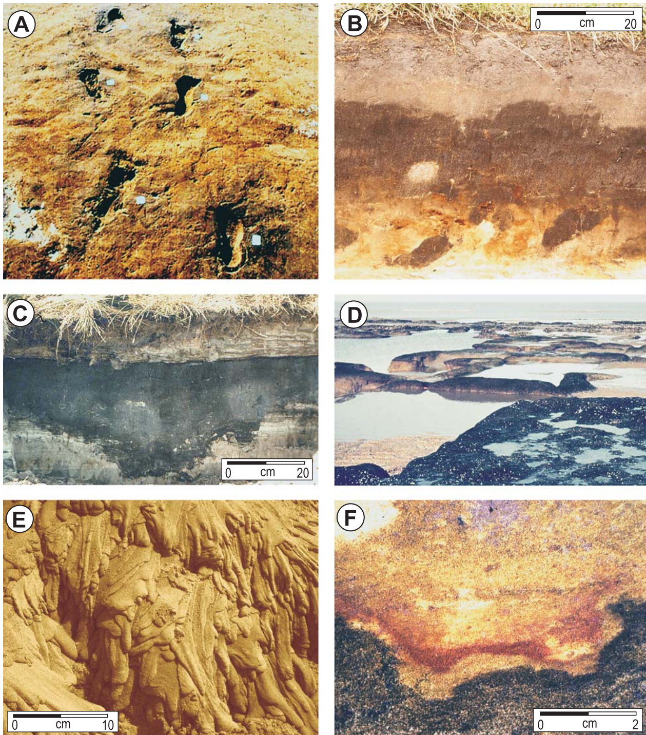
Fig. 22. Anthropogenic deformations. A: Foot steps left behind in fresh volcanic ash by Bronze Age people fleeing for an eruption of the Vesuvius volcano (Italy). B: Traces of prehistoric ploughing (producing dark pieces of a peaty podzol in the underlying - light-coloured - sands that did not undergo pedogenesis) in the coastal-dunes area of the western Netherlands. C: Pit dug by prehistoric Man as a waste-dump site. Surroundings of Marck (NW France). D: Remnants of Roman and Medieval peat digging exposed during low ebb tide off Raversyde (Belgium). Traces left by the spades used during the peat digging can still be found. E: Flow lobes on the slope of piled wet sands in the Jansen quarry at Uelsen (W Germany). F: SSDS intermediate between bioturbation and anthropoturbation: imprint made in Mediaeval times by cattle in a wet meadow near a farm. Coastal plain, NW France.
