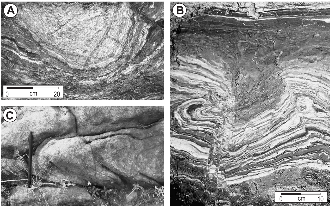
Fig. 7. Small causes can have significant results. A: 'Classical' load cast in the still unconsolidated, silt-rich subrecent Almere Member of the North Sea Formation (Noordoostpolder, The Netherlands). The loading did not cause any further deformations. B: Gravifossium near Emmeloord in the subrecent lagoonal Almere Member of the North Sea Formation near Emmeloord (The Netherlands). The deformation started as simple loading, but this occurred so quickly that a depression at the sedimentary surface resulted. This attracted new sediment, increasing the local weight, stimulating further loading. The load cast sunk ever deeper, until faulting took place along the almost vertical lateral boundaries. This faulting induced local stress systems that resulted in smaller deformations (both faults and faults). C: Simple processes like dragging of unconsolidated sediments can result in structures that are - without thorough analysis - difficult to distinguish from tectonic deformations in lithified rock. SSDS such as this dragging structure in the Palaeoproterozoic Chaibasa Fm. near Tata (E India) have therefore frequently been misinterpreted in the past.
