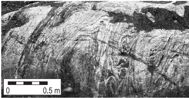
Fig. 3. Layer (right of centre) with soft-sediment deformations in the folded Precambrian basement of the Alstamalm sand quarry (S Sweden).
