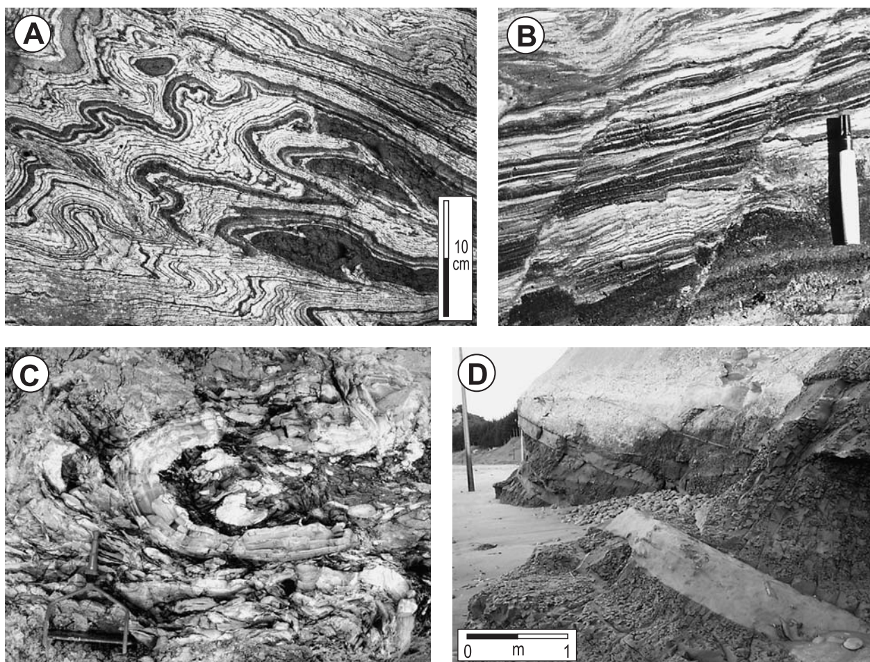
Fig. 4. The four principal types of deformations in soft sediments. A: Folds in a slump structure in the marine, calcareous Pleistocene Lisan Fm. (northern Arava, Israel). B: Faults formed in brackish lagoonal deposits of the subrecent Almere Member of the North Sea Formation while the sediment was still saturated with water. Surroundings of Emmeloord, The Netherlands. C: Breccia in the Pleistocene Ławki Formation. Bełchatów open-cast browncoal quarry (central Poland). Photo Beata Gruszka (Poznań). D: Intrusion of clay (layer with sharp upper and lower boundaries, from centre to lower right corner) into fine-grained Pliocene marine deposits, caused by the pressure exerted by the backwash of a giant tsunami (from Le Roux et al., 2008).
