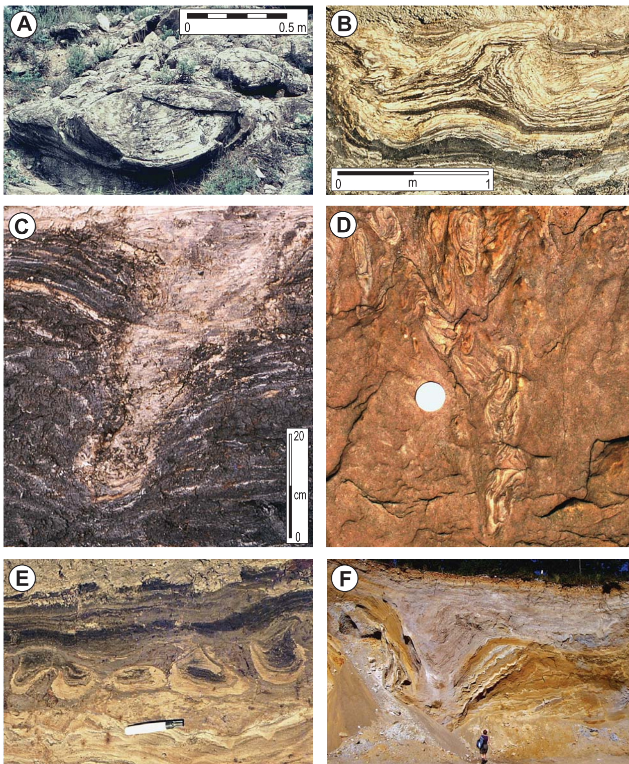
Fig. 16. Load casts and associated SSDS form a wide spectrum of structures, both in size and in shape. A: Loaded trough-shaped megaripples in the Cuisian/Lutetian Perarrua Fm. near Bellestar (Spain). B: Huge loadcasts within subrecent silty lagoonal sediments (North Sea Formation) in the reclaimed Noordoostpolder (The Netherlands). C: Narrow loadcast of some 10 cm wide and some 50 cm deep. Location as Figure 16B. D: Extremely developed, loadcast in the Palaeoproterozoic Chaibasa Fm., near Dhalbhum Gar, E India. The loadcast must have development during several phases, as younger loadcasts deform and push further down older loadcasts. E: Pseudonodules, reflecting an entirely broken-up layer of fine sand. Location as Figure 16B. F: Large-scale gravifossom in Weichselian glaciofluvial sands and gravels in a quarry near Ryssjön (S Sweden).
