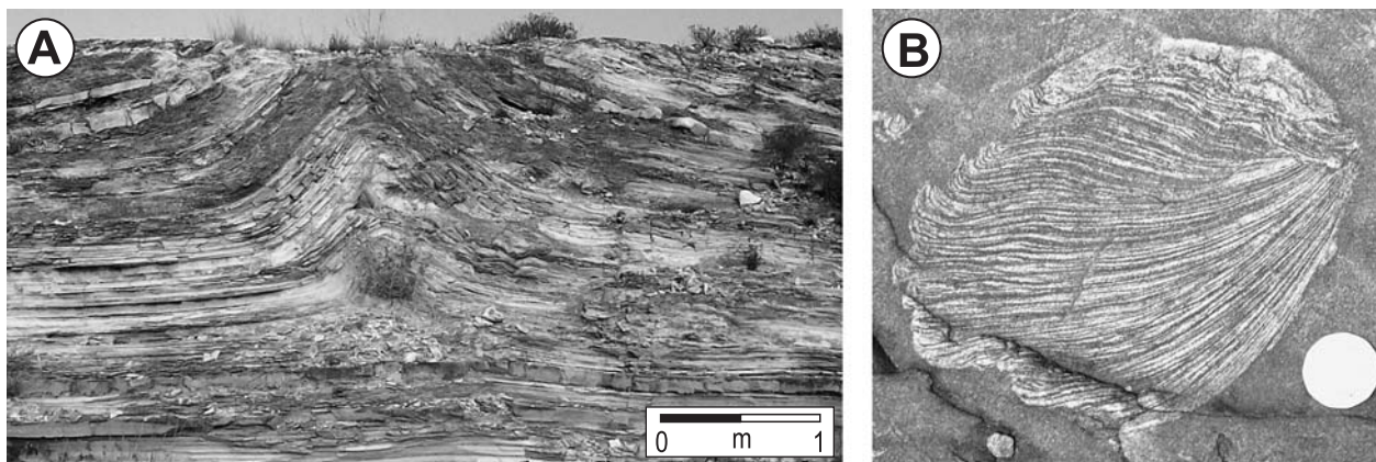
Fig. 30. SSDS of enigmatic origin. A: Structures in the Late Cretaceous Boquillas Fm., along Highway I-90 in the neighbourhood of Del Rio (Texas, U.S.A.). The structures have been described as tepee structures (Johnston, 1983) and later as a result of expansion due to recent caliche forming (Lock et al., 2001), but none of these explanations is convincing. B: More or less rounded structures occur fairly frequently as isolated 'balls' in the Palaeoproterozoic Chaibasa Fm. near Dhalbhum Gar (E India), but their shapes do not support an interpretation as unconsolidated fragments that became rounded by rolling over the bottom of the shallow sea. The internal structure of the various individual balls is identical. No satisfactory explanation of their genesis has been put forward so far.
