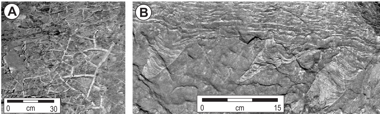
Fig. 28. Presumed synaeresis cracks. A: Bedding plain in rocks of unknown age in Peru, showing cracks that form irregular patterns that do not resemble desiccation cracks and that are ascribed to synaeresis. Photo G.R. Morton. B: Cross-section through infilled irregular cracks in the shallow-marine part of the Palaeoproterozoic Chaibasa Fm. (Singhbhum area, India) that might represent synaeresis cracks.
