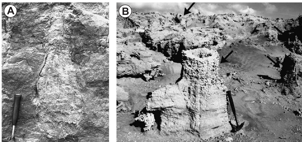
Fig. 20. Sediments affected by soil conditions due to plant roots. A: Reduction zone around roots in (oxidated) Tertiary greensands at Herentals (Belgian Ardennes). B: Megarrhizoliths (indicated by arrows) in a Pleistocene dune field on Gran Canaria (Spain). Photo Ana Alonso-Zarza (Madrid).
