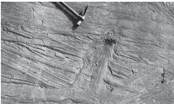
Fig. 19. Groove casts, one of which shows the object that caused the structure at its end. Flysch facies of the San Vicente Fm. near Atiat (Pyrenees, Spain).
