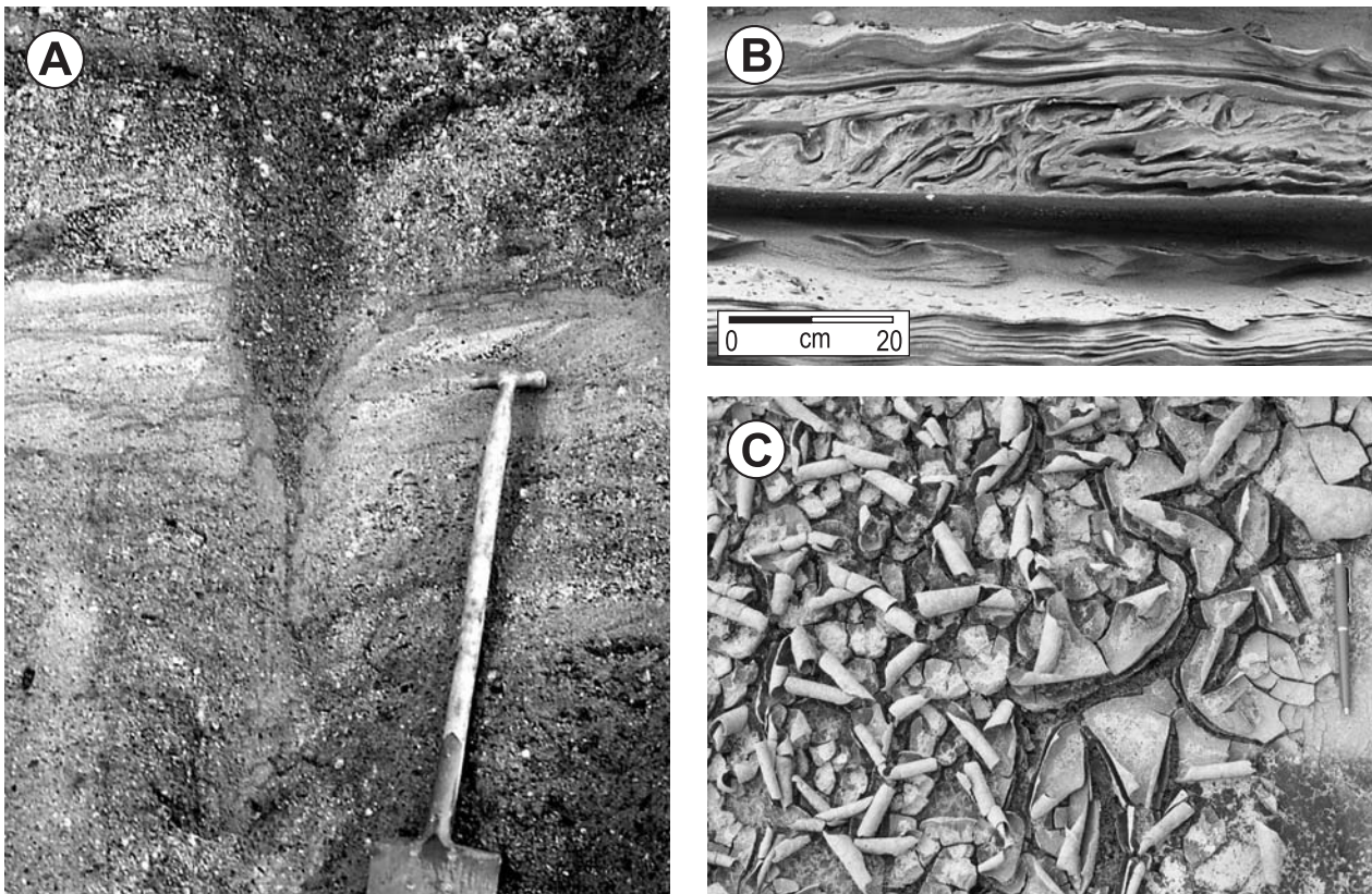
Fig. 6. Soft-sediment deformation structures of different sizes. A: Large-scale frost wedge penetrating several Saalian glaciofluvial layers, including a gravel bank cemented by iron oxides and hydroxides at Balderhaar (Germany). B: Meso-scale deformation affecting an entire layer of spouted sand. C: Small-scale deformations in the form of curled-up clay, caused by differential contraction between the lower, somewhat sandy parts and the more clayey upper parts of a fine-grained layer.
