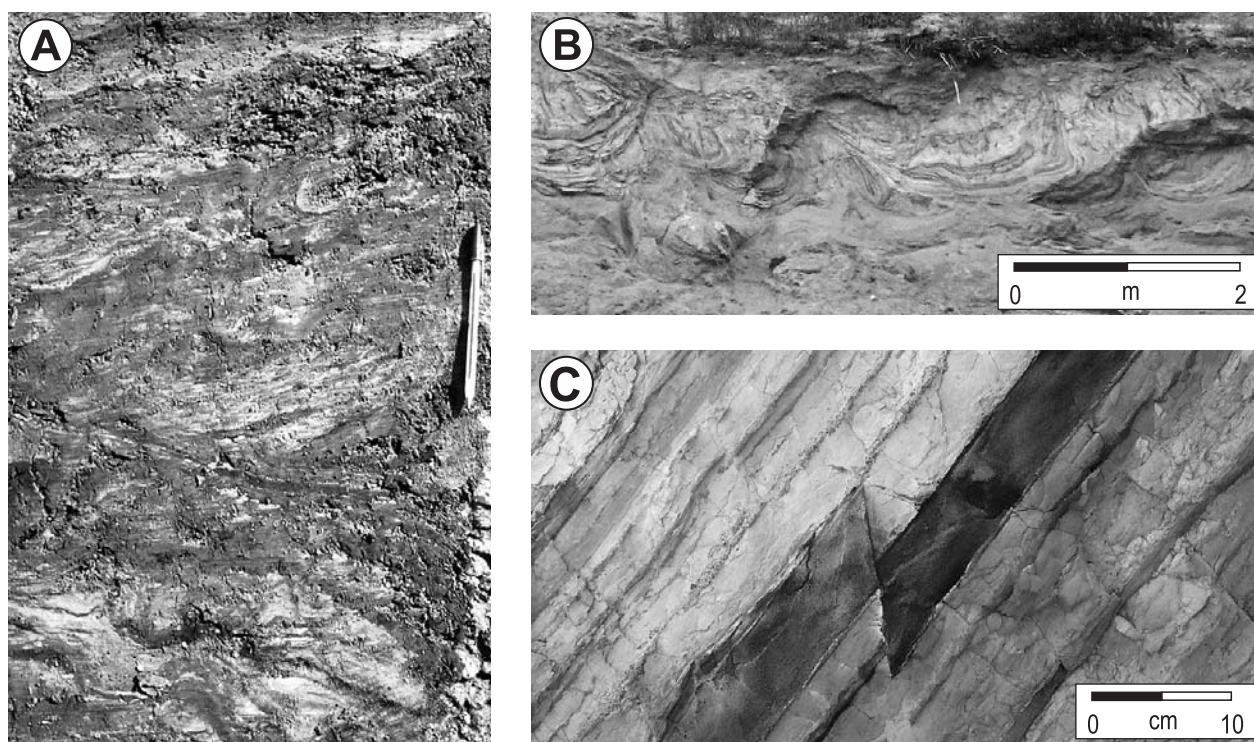
Fig. 5. The three main states of unconsolidated sediments during deformation. A: Partial disappearance of the primary structures in the silt-rich upper part (1250–1600 AD) of the lagoonal Almere Member of the North Sea Formation (Noordoostpolder, The Netherlands), due to partial liquefaction (fluidized state). B: Cryoturbation in the upper layer (Pleistocene) of the Ryssjön quarry (S Sweden), indicating plastic behaviour of the sediment during deformation. C: Synsedimentary fault (indicating brittle behaviour) in the Miocene Misaki Fm. on the Miura Peninsula (Japan). The area underwent frequent seismic activity.
