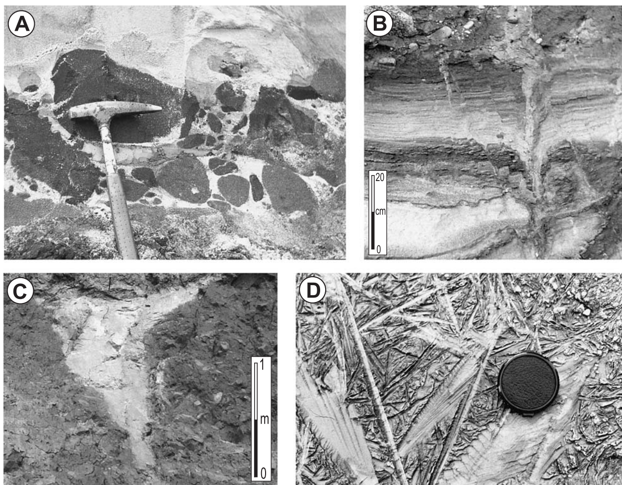
Fig. 24. Thermoturbations. A: Rounded pebbles of Miocene browncoal in the Neurather Sand, formed by transport in frozen condition during the Pleistocene. Morken open-cast browncoal mine (W Germany). B: Frost fissure in the Beuningen Layer at Getelo (Germany). C: Frost wedge in Weichselian sediments at Ścinawka Średnia (Poland). D: Imprints of ice crystals (view from above) in a muddy soil near Ginzling (Austria).
