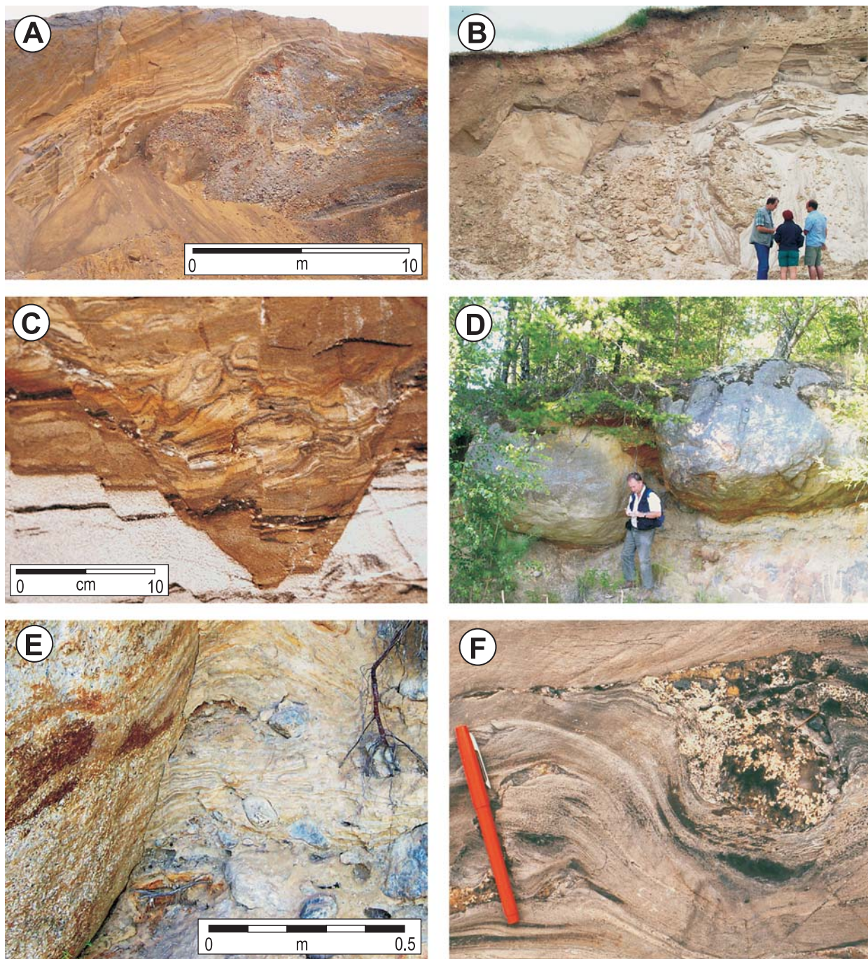
Fig. 23. Glaciturbations are mainly produced by pressure (e.g. in ice-pushed ridges), tension (e.g. occurring when ice under or alongside a glacial deposit melts away), or by stones that fall down in water (e.g. from an ice raft or the roof of a subglacial channel). A: Large-scale glacitectonic deformations as a result of pressure in a sand quarry near Hummelhaga (S Sweden). B: Blocks consisting of esker sediments formed by relaxation (de facto tension) after the ice walls had melted away. Surroundings of Wielowiczek (Poland). C: Graben-like deformation (commonly called 'dead-ice structure') in fluvio-glacial sands due to melting (de facto resulting in tension) of buried dead-ice underneath. Belchatow opencast mine (central Poland). D: Huge dropstones in a quarry near Axelsberg (S Sweden). The unconsolidated sediment underneath is relatively slightly deformed, possibly because the stones fell on the slightly inclined hard (Precambrium) substratum and then toppled over. Photo: Amir Mokhtari Fard (Bromma). E: Intense deformation between the two huge dropstones of Figure 23D, possibly caused when the second stone tumbled over on the substratum towards the first one, pressing up the material in between them. F: Small dropstone in Huronian glaciomarine sediments, causing relatively slight deformation of the underlying fine-grained sediment (Alberta, Canada).
