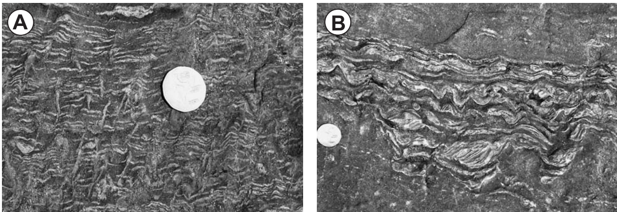
Fig. 10. SSDS in seismites of the shallow-marine part of Palaeoproterozoic Chaibasa Fm. near Dhalbhum Gar (E India). A: Numerous small-scale clastic dykes indicate sudden attempts of pore water to escape, probably under the influence of an earthquake-induced shock wave. B: Strongly disturbed seismite with identical granulometry as the under- and overlying layers.
