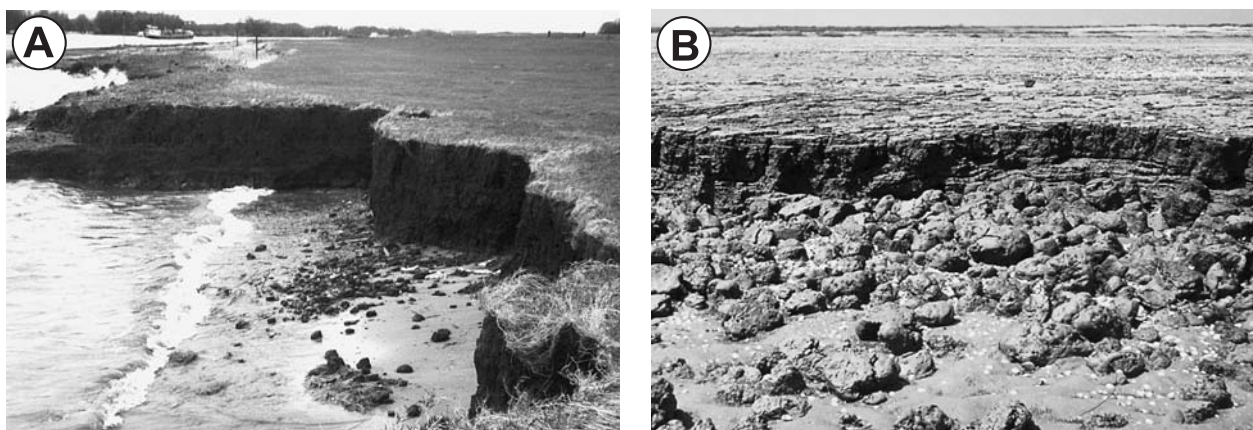
Fig. 17. Deformation of clay balls due to current and wave action. A: Undercutting of natural levees during high-discharge periods cause clay balls to be formed at the foot of the 'cliff'. The clay masses that have fallen down from the cliff become rolled up during transport by the river. Waal River between Oosterhout and Slijk-Ewijk (The Netherlands). B: Clay balls at the foot of a salt-marsh cliff become rolled up mainly by to-and-fro movements under the influence of wave action. Land van Saeftinghe, SW Netherlands.
