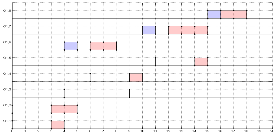
Figure 3. Admissible solution for time horizon H = \{0, 1, \dots, 20\}
