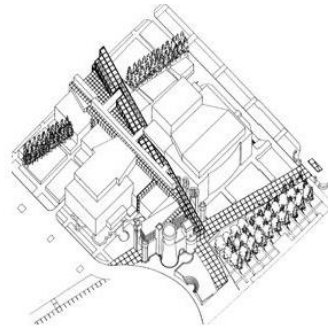
12. P. Eisenman, Wexner Center for the Visual Arts , The Ohio State University, Columbus, 1983-1989 za: A Center for the Visual Arts. The Ohio State University Competition , red. P. Arnell, T. Bickford, New York 1984, s. 118.
