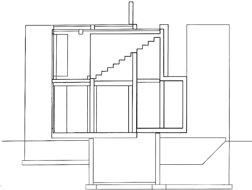
6. P. Eisenman, House VI , 1973 za: Eisenman Architects. Selected and Current Works , red. S. Dobney, Mulgrave 1995, s. 42.
