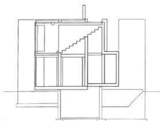
6. P. Eisenman, House VI , 1973 za: Eisenman Architects. Selected and Current Works , red. S. Dobney, Mulgrave 1995, s. 42.
