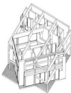
4. P. Eisenman, House III , 1969 za: M. Gandelsonas, From Structure to Subject: The Formation of an Architectural Language , „Oppositions” 1979, nr 17, s. 10, rys. 4.
